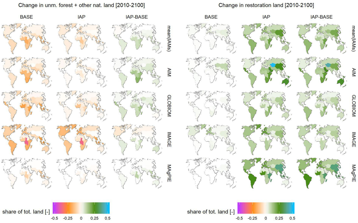
Extended Data Fig. 5 | Spatial patterns of projected habitat loss and restoration by 2100. Data are shown for the BASE and IAP scenarios and the difference (IAP – BASE), and are shown as the mean across IAMs (top) and separately for each of the four IAMs (AIM, GLOBIOM, IMAGE, MAGPIE).
