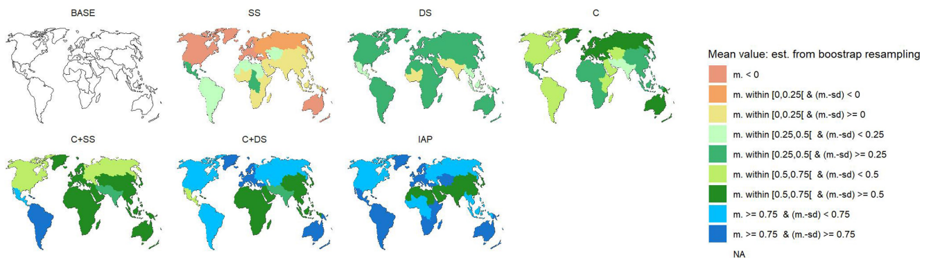
Extended Data Fig. 7 | Spatial patterns of the date of peak loss in the twenty-first century and the share of avoided future peak loss. a, b, Across the 17 IPBES subregions, individual maps show, for each region and for each of the seven scenarios, the mean value of the date of peak loss in the twenty-first century (a) and the share of avoided future peak loss (b). Means were estimated
